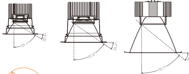
View Cut off Angle
