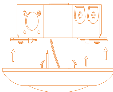
Surface Mount
