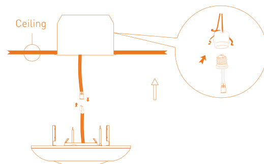
Recessed Mount
